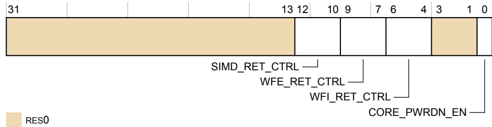
Figure B2-33 CPUPWRCTLR_EL1 bit assignments
