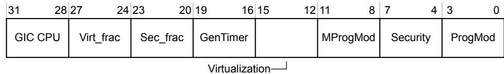
Figure B2-68 ID_PFR1_EL1 bit assignments
