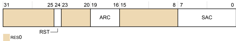
Figure D10-61 TRCSSCCR0 bit assignments
