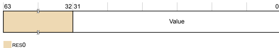
Figure D10-8 TRCCIDCVR0 bit assignments
