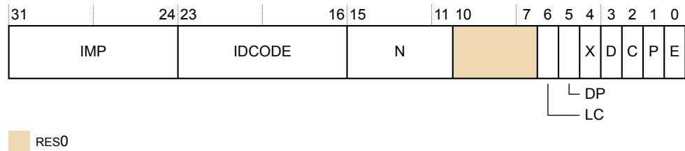
Figure D4-3 PMCR bit assignments
