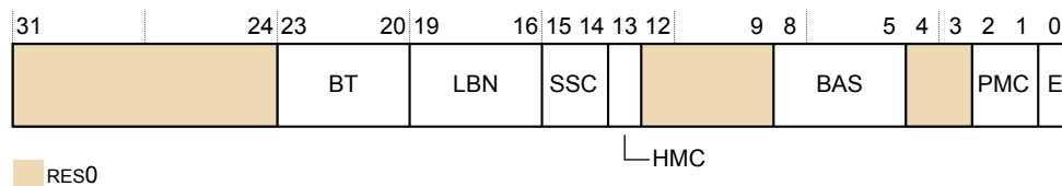
Figure D2-1 DBGBCRn_EL1 bit assignments
