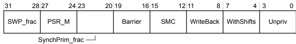
Figure B2-59 ID_ISAR4_EL1 bit assignments
