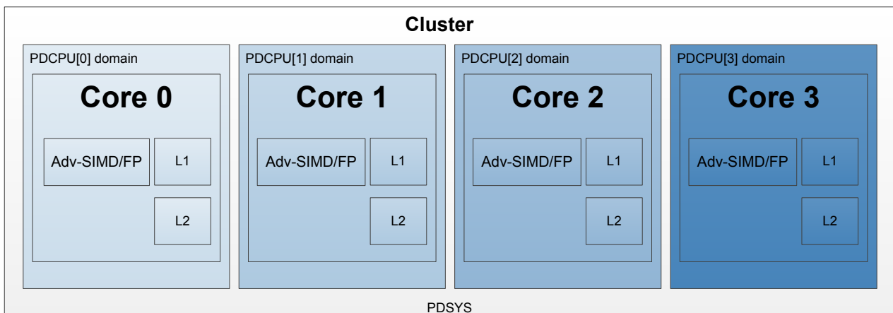
Figure A4-3 Cortex-A77 power domains at deimos_core level
