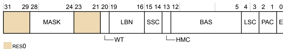
Figure D2-3 DBGWCRn_EL1 bit assignments
