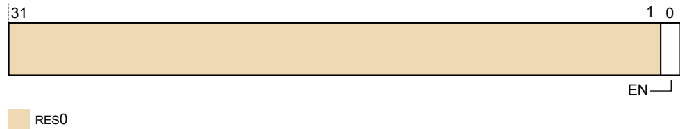
Figure D8-2 MUSERENR_EL0 bit assignments
