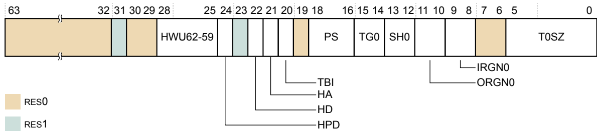
Figure B2-84 TCR_EL2 bit assignments
