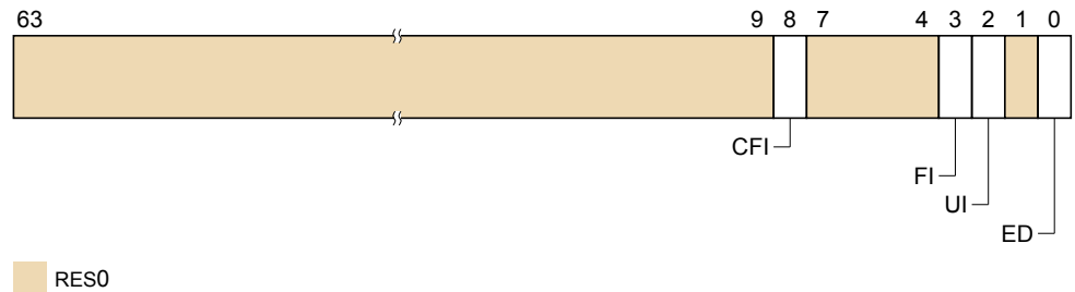
Figure B3-2 ERR0CTLR bit assignments
