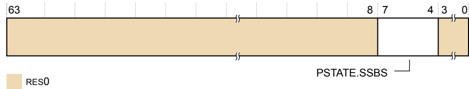
Figure B2-52 ID_AA64PFR1_EL1 bit assignments
