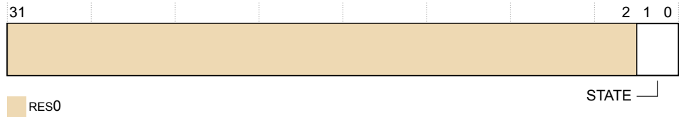
Figure D10-60 TRCSEQSTR bit assignments
